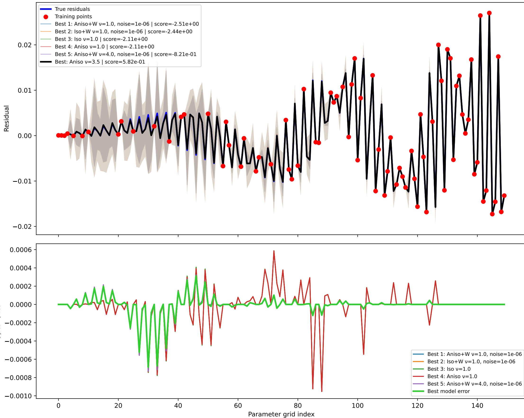
GPR kernel comparison node=23 RMSE=1.153e-04, train RMSE=9.182e-12
